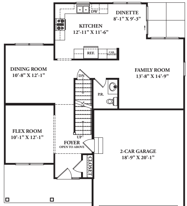
FIRST FLOOR 943 SQ. FT.
