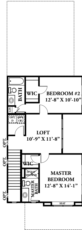
SECOND FLOOR 797 SQ. FT.
