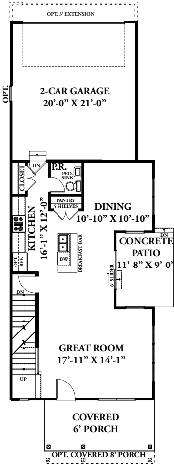
FIRST FLOOR 785 SQ. FT.
