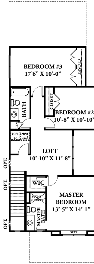
OPT. SECOND FLOOR 1,007 SQ. FT.
