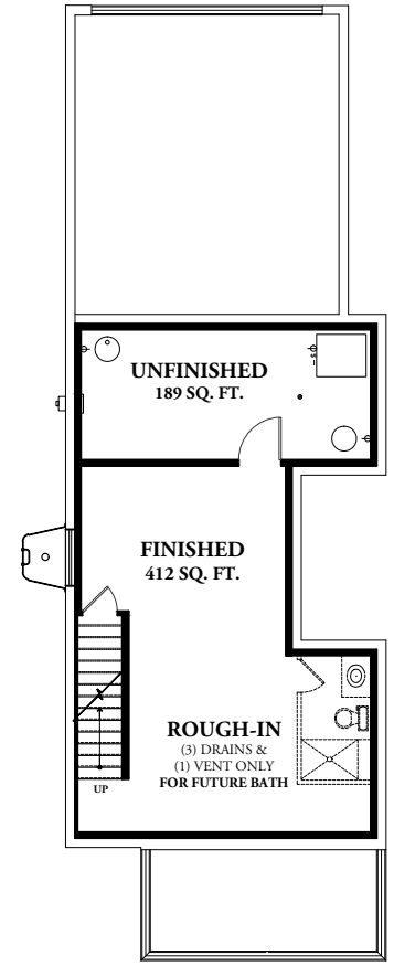
OPT. PARTIAL FINISHED BASEMENT 412 SQ. FT.
