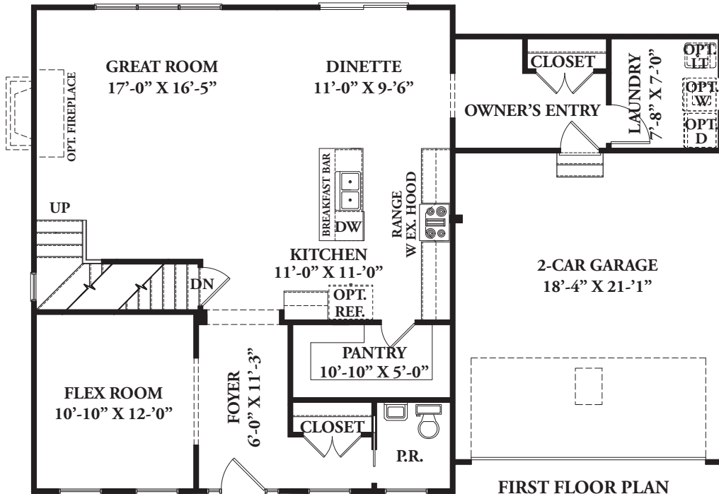
FIRST FLOOR PLAN 1,105 SQ. FT.
