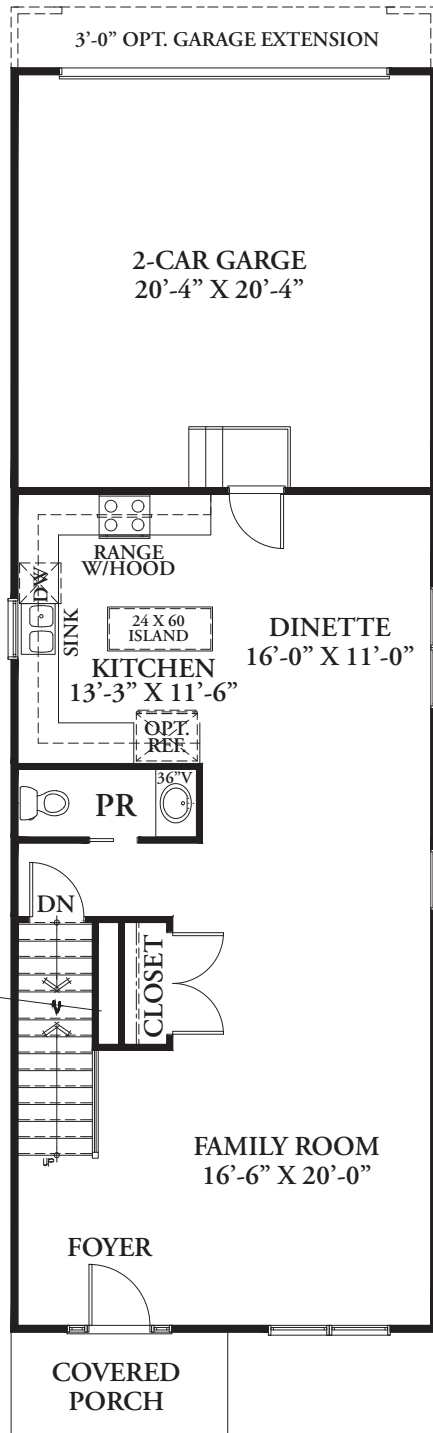
FIRST FLOOR 873 SQ. FT.
