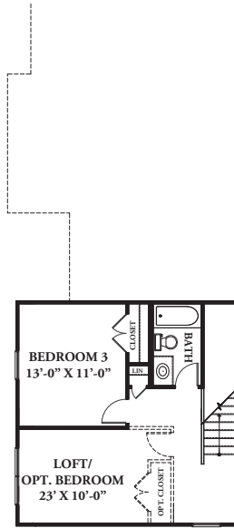
ELEVATION II SECOND FLOOR 457 SQ. FT.
